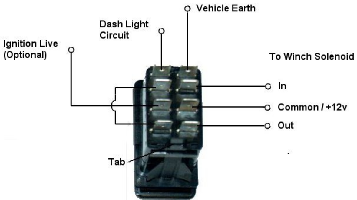
Using a Carling DPDT Switch to control a winch.
